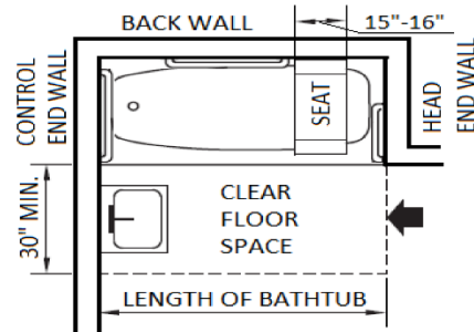
(b) REMOVABLE SEAT IN TUB - SIDE APPROACH
