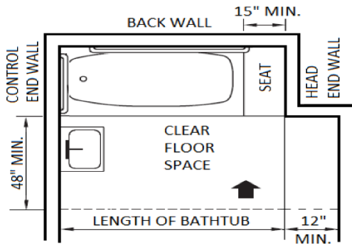
(c) PERMANENT SEAT IN TUB - FRONT APPROACH
