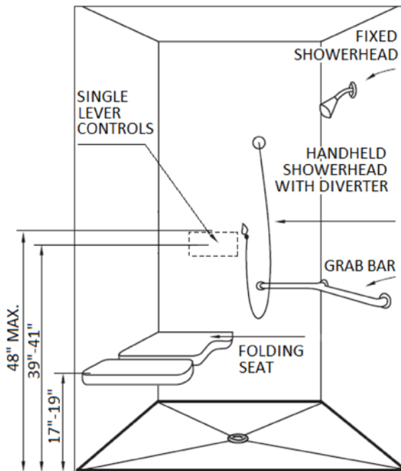
(b) 42" x 48" ROLL-IN SHOWER
