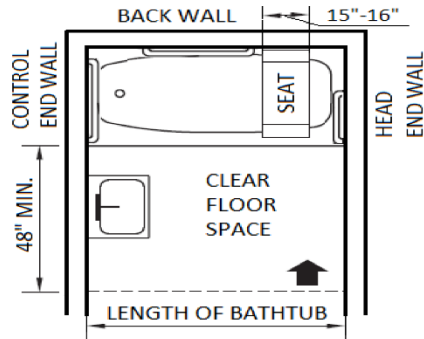
(a) REMOVABLE SEAT IN TUB - FRONT APPROACH
