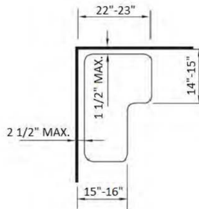
(b) SHOWER SEATS
