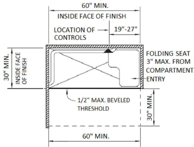
(a) 60" x 30" ROLL-IN SHOWER
