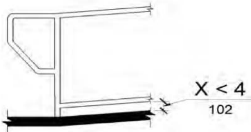
FIGURE 11B-405.9.2 CURB OR BARRIER EDGE PROTECTION
