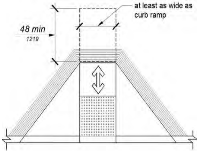
FIGURE 11B-406.5.3 LANDINGS AT THE OF CURB RAMPS
