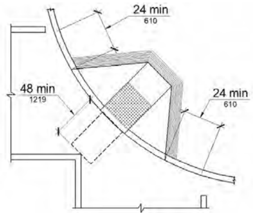
FIGURE 11B-406.5.10 DIAGONAL OR CORNER TYPE CURB RAMPS
