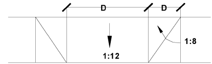
CURB RAMP
