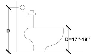
DETAIL - WATER CLOSET
