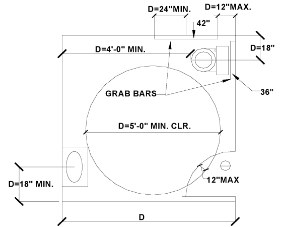
PLAN VIEW - TOILET ROOM
