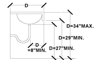
DETAIL - LAVATORY
