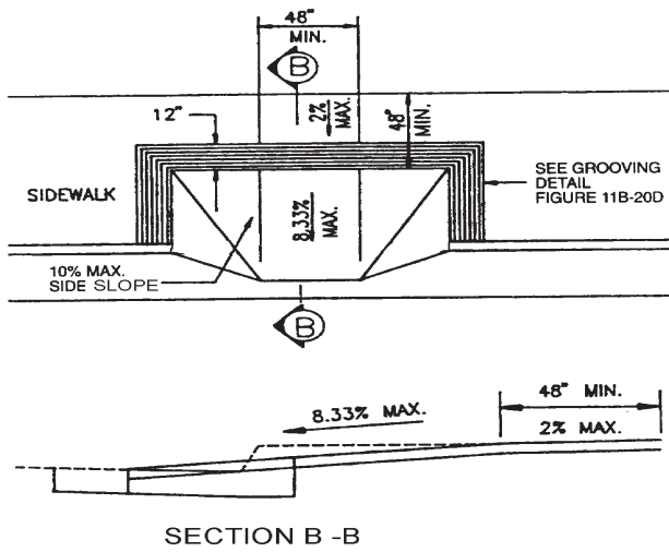
FIGURE 11B -19C -CURB DETAILS
