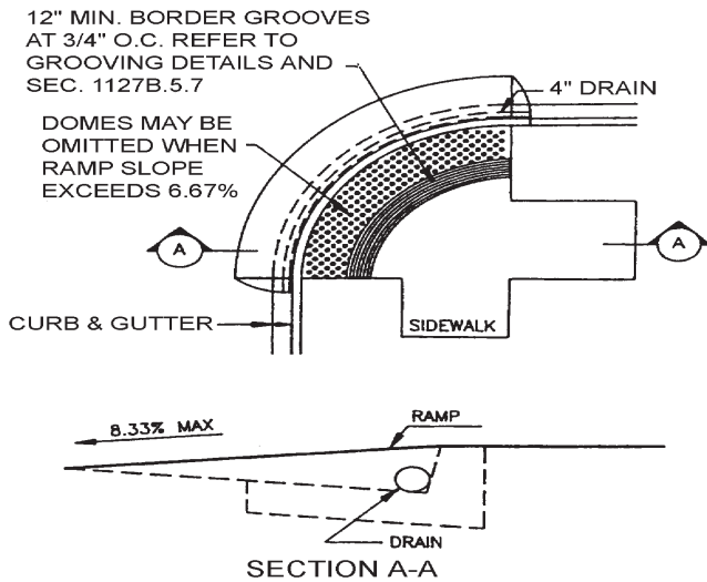
FIGURE 11B -19A -CURB DETAILS
