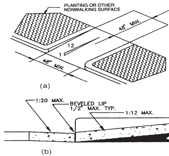
FIGURE 11B -21 -RETURNED CURB STYLE
