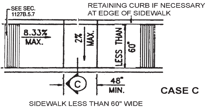
FIGURE 11B -20 A -CURB DETAILS
