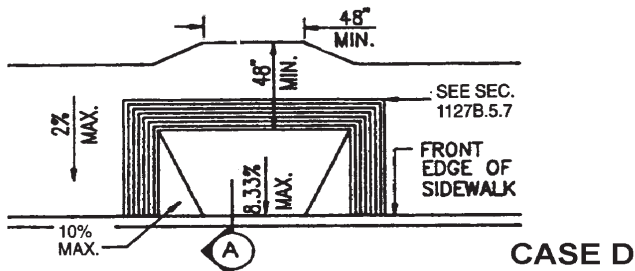
FIGURE 11B- 20B -CURB DETAILS
