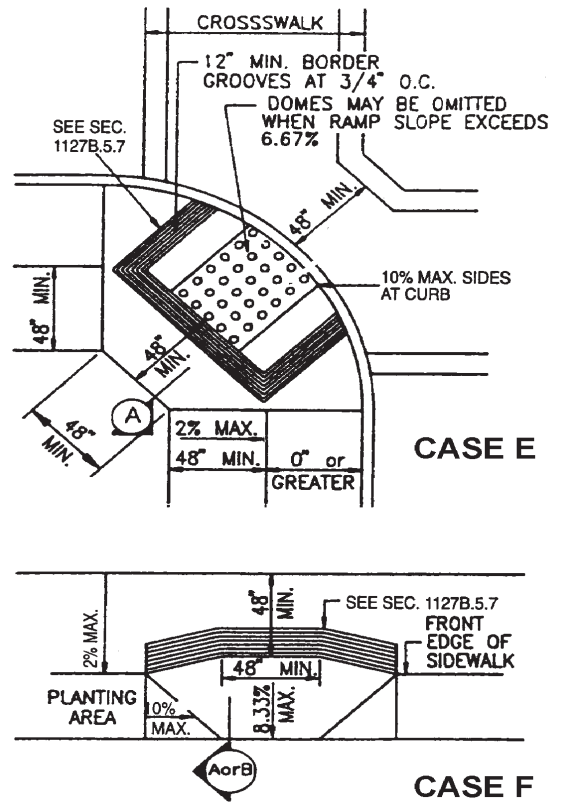
FIGURE 11B -20C -CURB DETAILS
