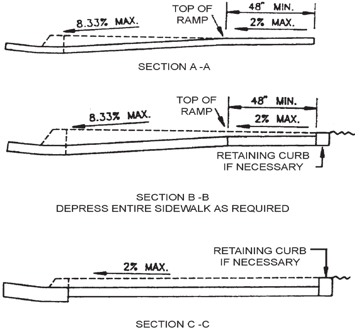
FIGURE 11B -20E -CURB SECTIONS
