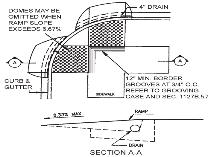
FIGURE 11B -19B -CURB DETAILS
