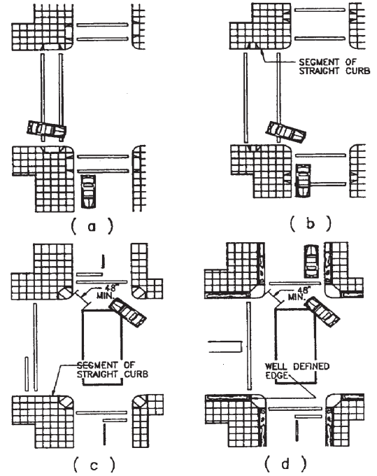
FIGURE 11B -22 -CURB RAMPS AT MARKED CROSSING
