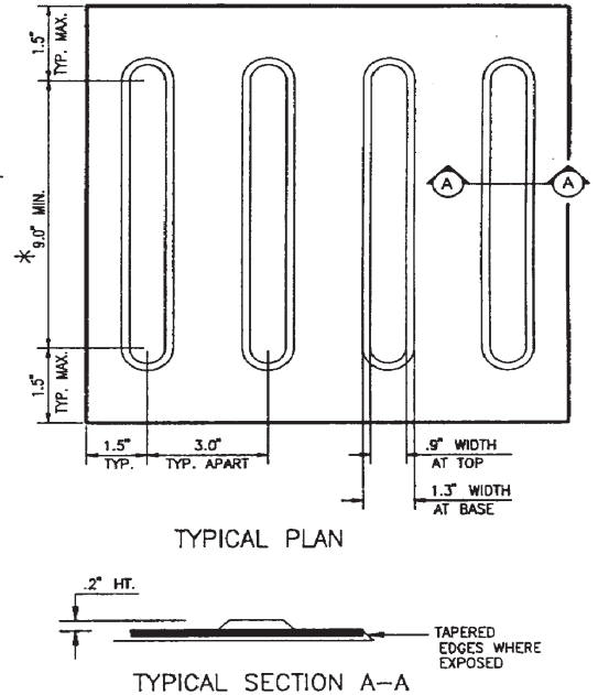
FIGURE 11B -23B DIRECTIONAL BARS
