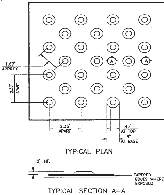
FIGURE 11B -23A TRUNCATED DOMES
