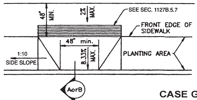
FIGURE 11B -20C -CURB DETAILS
