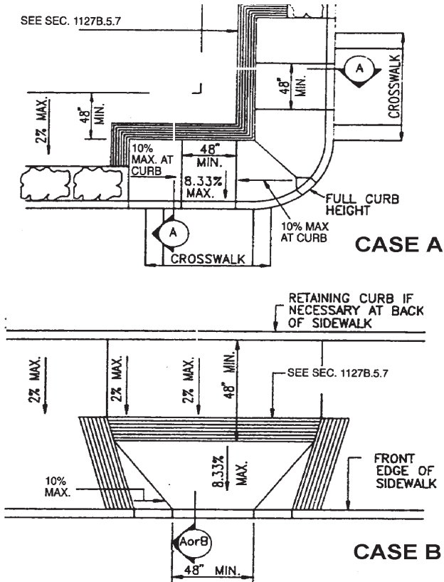
FIGURE 11B -20 A -CURB DETAILS
